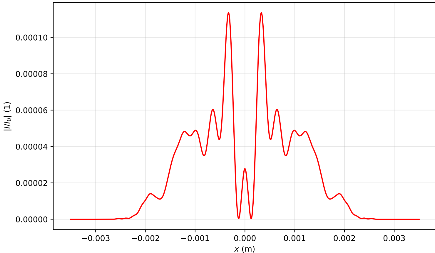
Intensity profile I(x, y = 0, z = 1.274)/I_0 , P_{in}=9.0P_{cr} , artificial time
